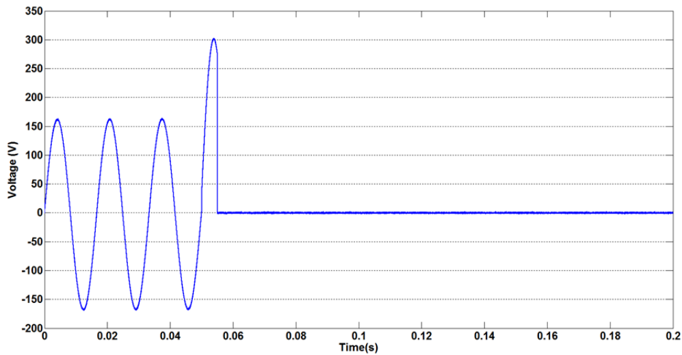
Figure 8: Voltage after inverters are tripped.
