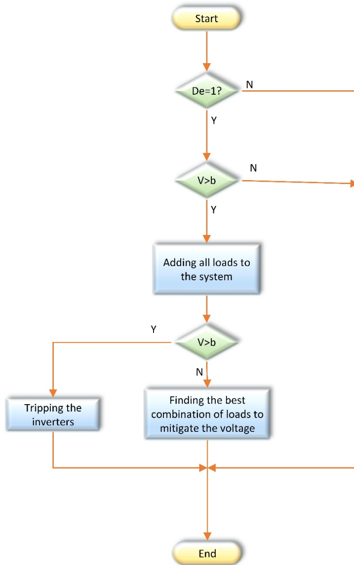
Figure 7: TOV mitigation logic using added loads ( b=1.1V_g ).
